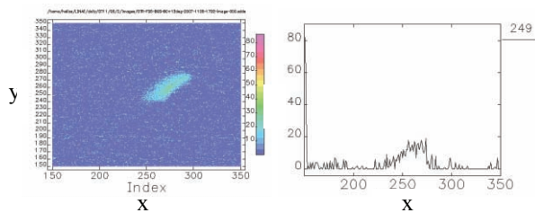
Figure 4: OTR beam image (left) and horizontal profile (right) sampled through distribution after BC with L2 phase = 12 degrees, close to minimum compression.
