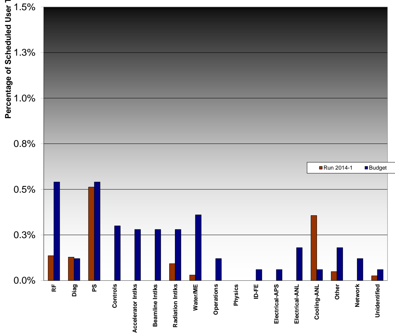
Run 2014-1 Downtime by System January 28 - April 21, 2014 Scheduled User Time = 1679 hours User downtime= 22.32 hours
