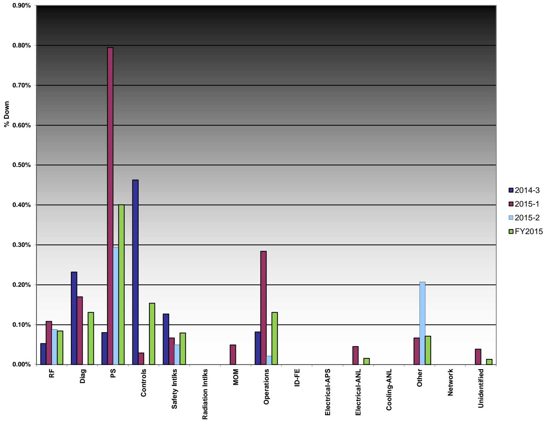
FY 2015 Downtime by System Data through Run 2015-2
