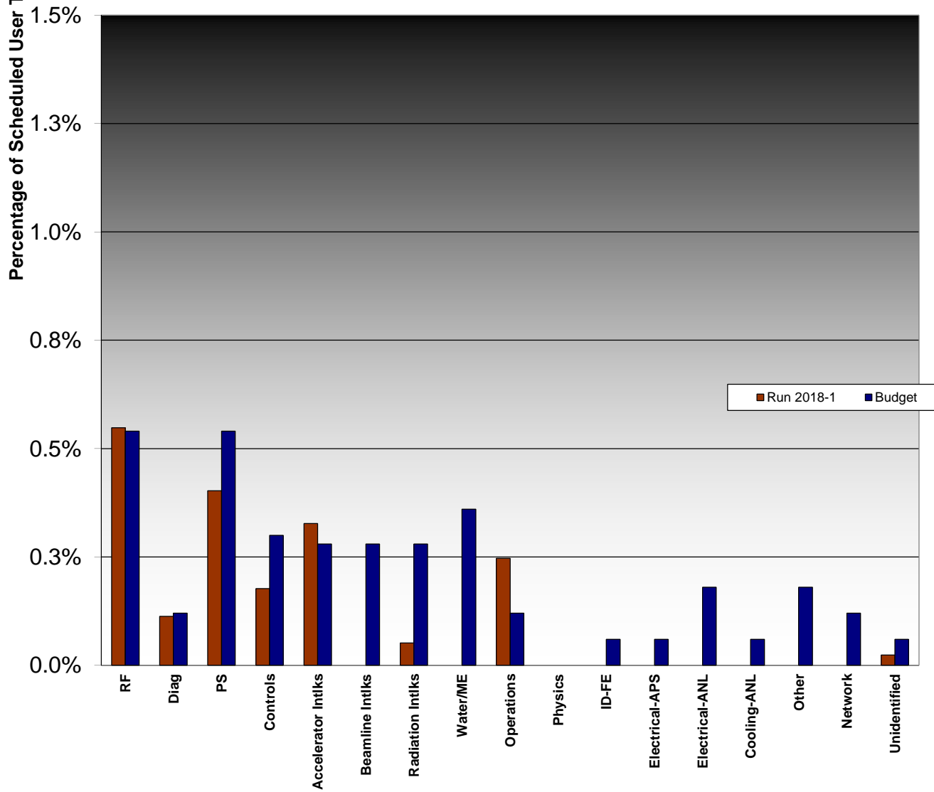
Run 2017-1 Downtime by System January 30 - April 24, 2018 Scheduled User Time = 1744 hours User downtime = 32.85 hours
