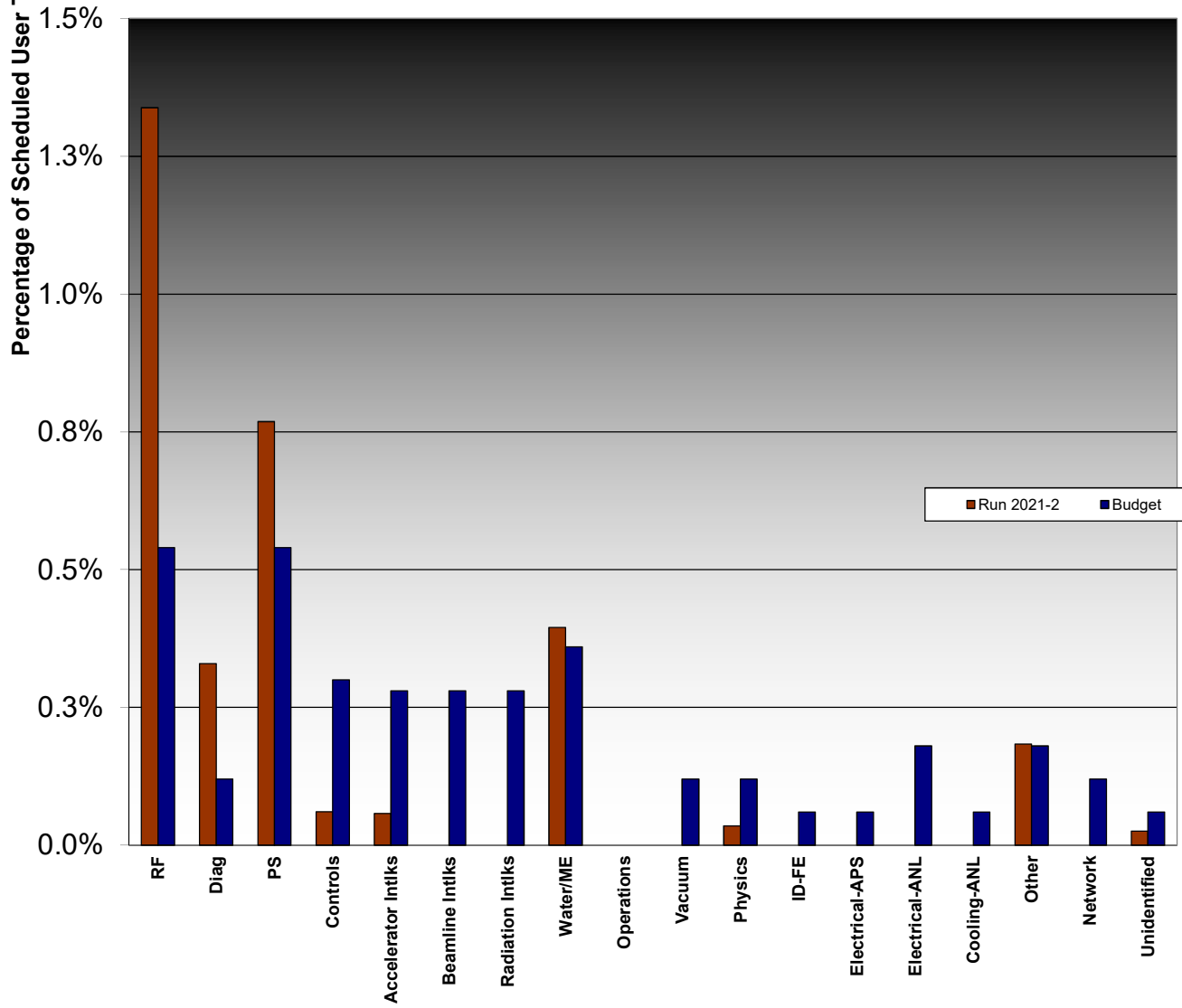
Run 2021-2 Downtime by System June 2 - September 30, 2021 Scheduled User Time = 1624 hours User downtime= 51.87 hours
