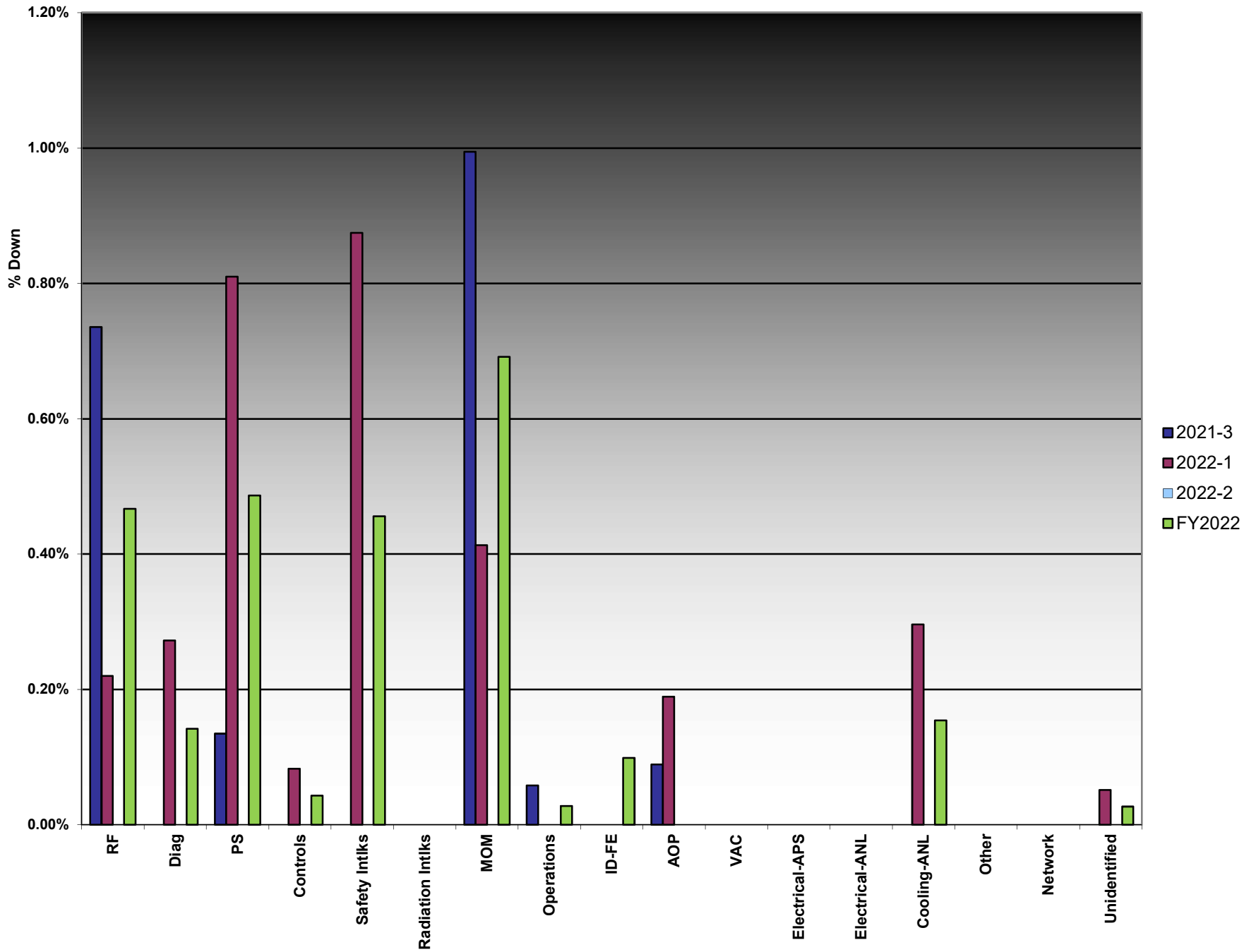
FY 2022 Downtime by System Data through Run 2022-1
